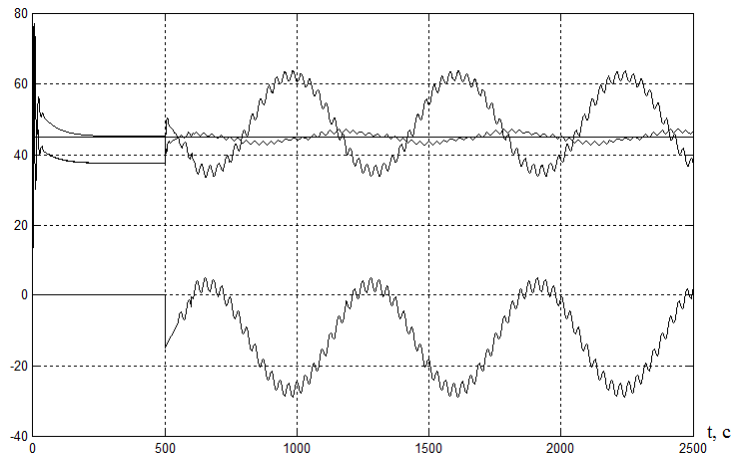
Fig. 5 – Modeling results control system ( K = 1.3 , \tau = 0 , T = 2 sec)
