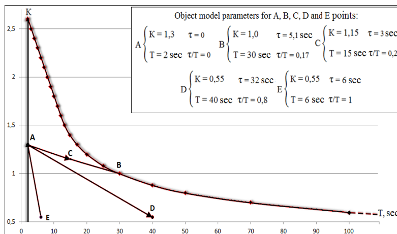
Fig. 3 – The normal working area of the suggested hybrid regulator (coordinate system T – K)
