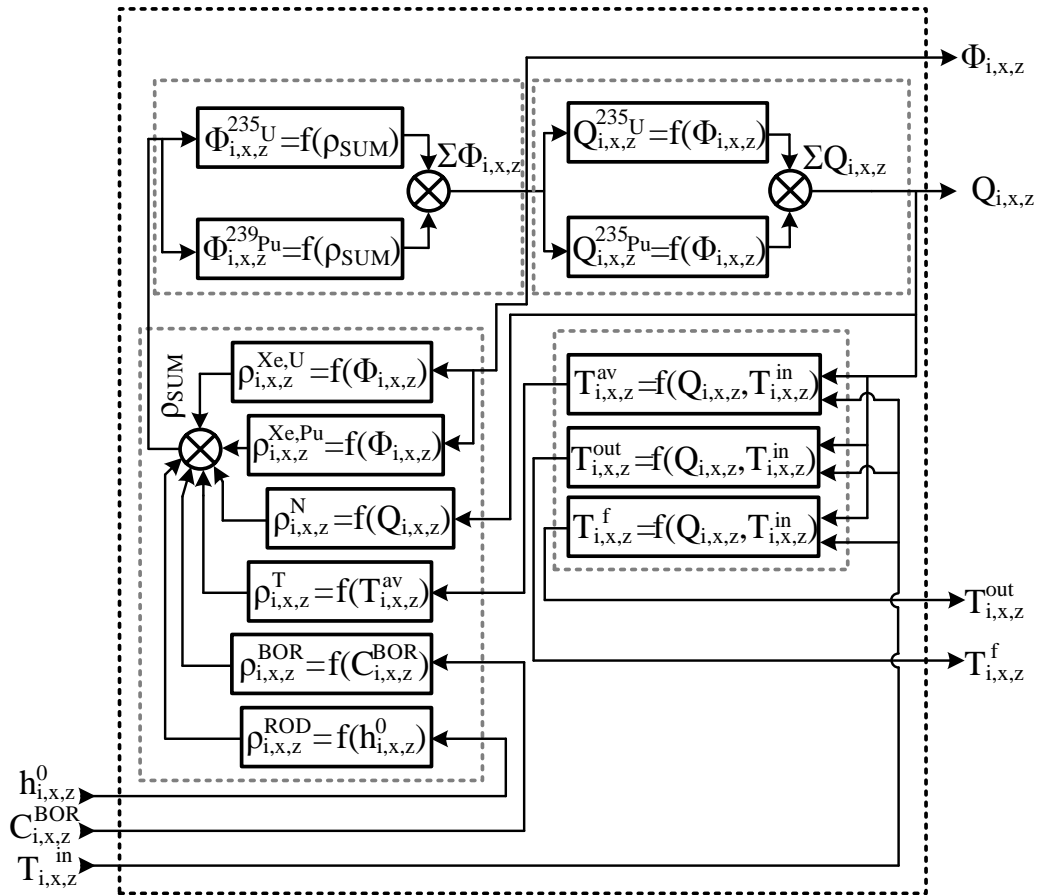
Fig. 1 - Diagram of the simulation model proposed RC unit cell
