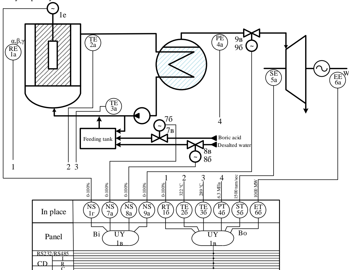
Fig. 4 – Advanced diagram of two automated control programs with constant average water temperature of the 1 st circuit and with constant steam pressure in the 2 nd circuit
