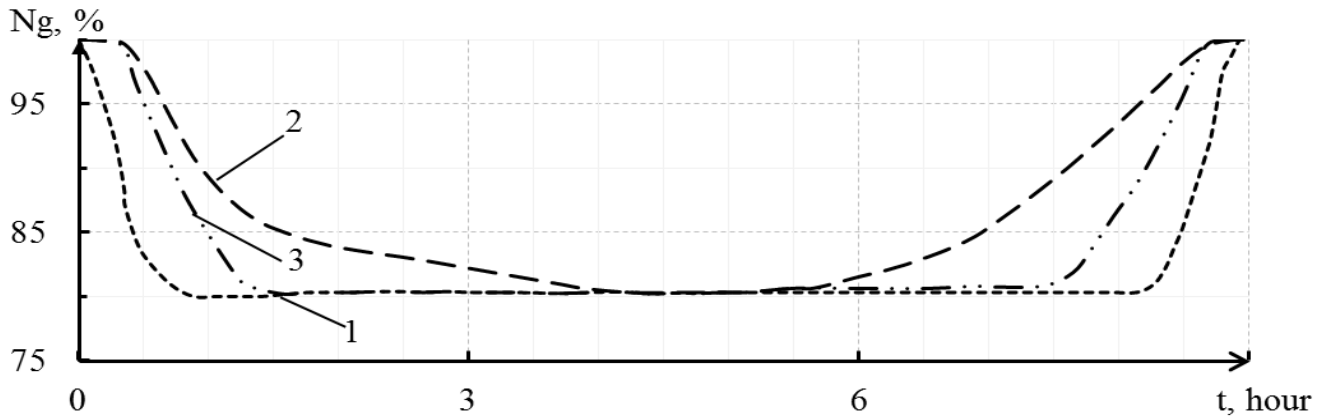
1 - improved ACS with constant average water temperature of the 1 st circuit; 2 - improved ACS with constant average water temperature of the 1 st circuit, which is designed by Tsyselska T.A.; 3 – primary ACS with constant average water temperature of the 1 st circuit
