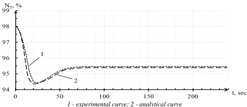
Fig. 3 - Effect of the control rods, which are introduced in the RC, to change of the neutron reactor power
