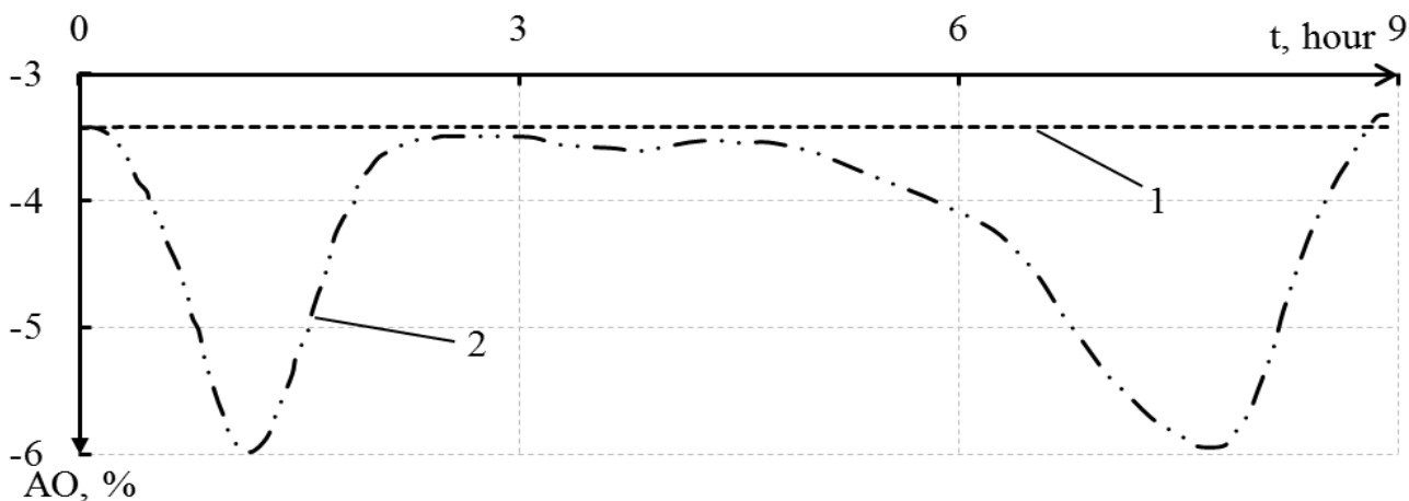
1 - improved ACS with constant average water temperature of the 1 st circuit; 2 – primary ACS with constant average water temperature of the 1 st circuit
