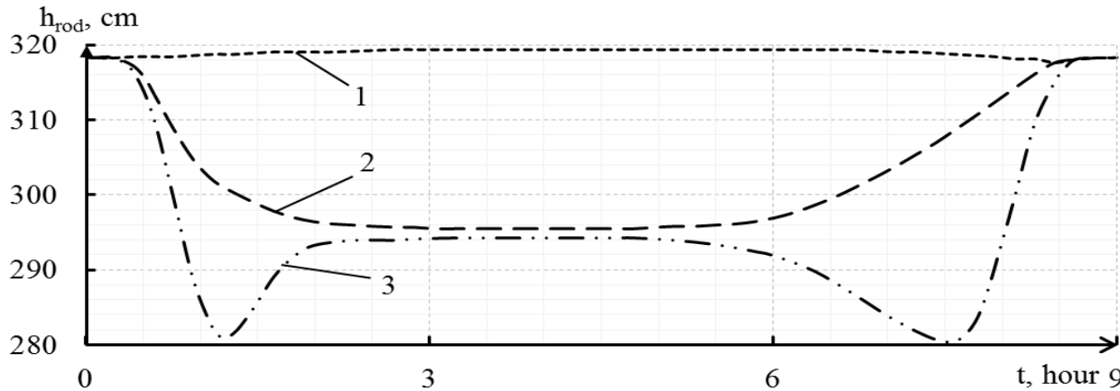
1 - improved ACS with constant average water temperature of the 1 st circuit; 2 - improved ACS with constant average water temperature of the 1 st circuit, which is designed by Tsyselska T.A.; 3 – primary ACS with constant average water temperature of the 1 st circuit
