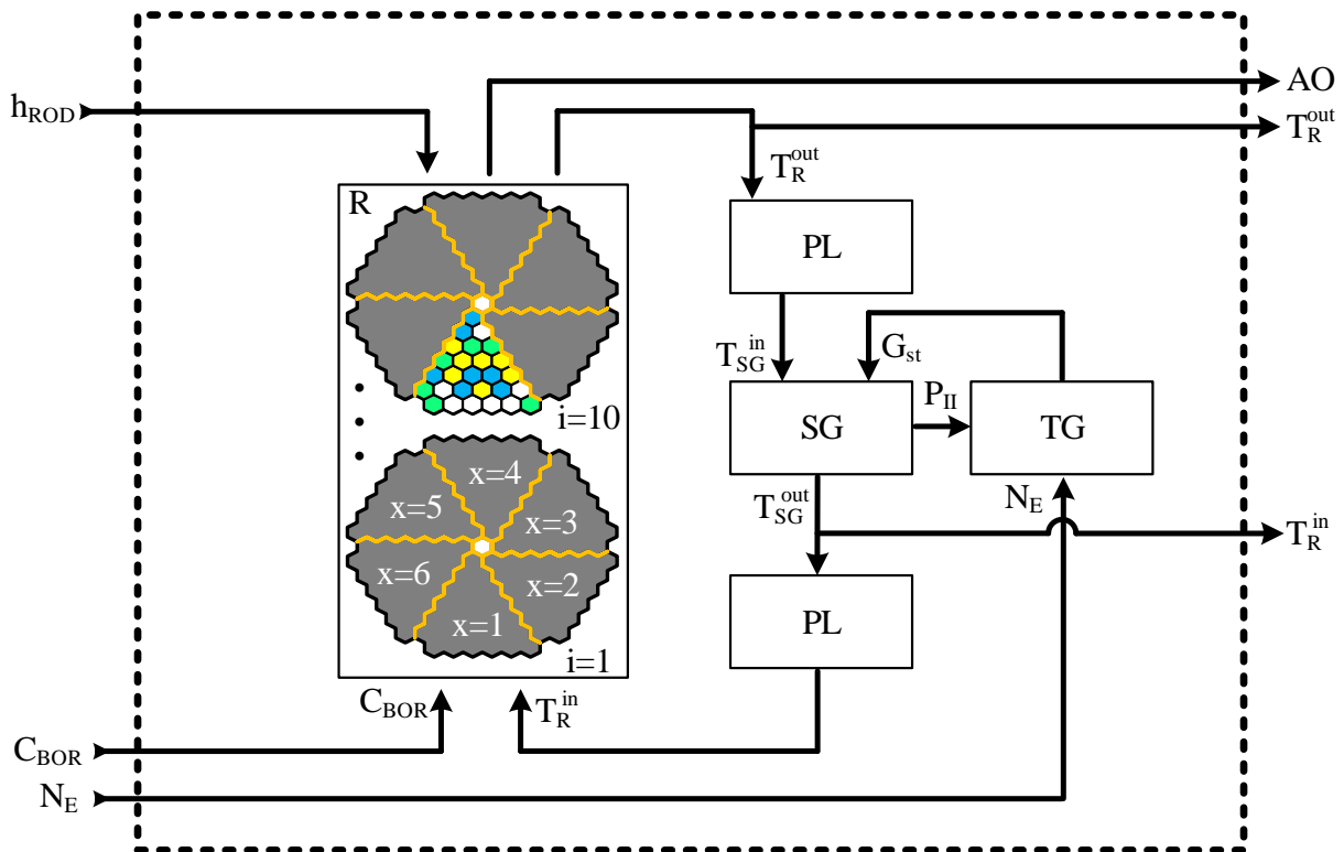
Fig. 2 - NPP simulation model VVER-1000 with allocated RC and without controllers
