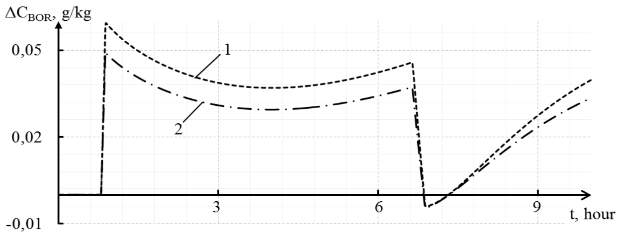
1 - control program with constant average water temperature of the 1st circuit; 2 - control program with constant steam pressure in the 2nd circuit
