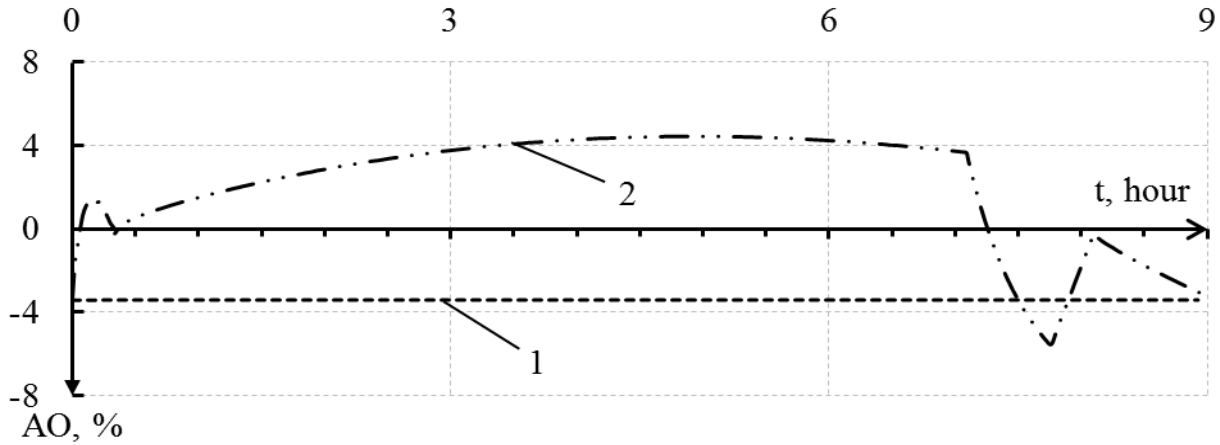
1 - improved ACS with constant steam pressure in the 2nd circuit; 2 - primary ACS with constant steam pressure in the 2nd circuit
